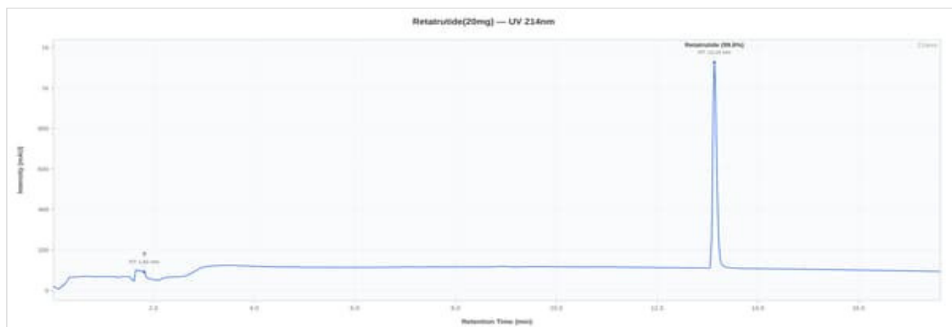
GLP3-RETA 20mg - 124-03-SM: UV chromatogram, 214 nm
